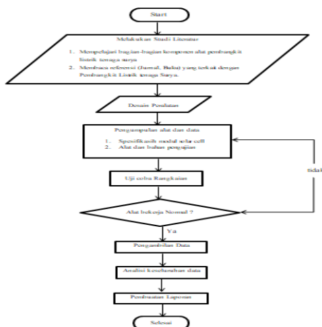
Gambar 5 Flowchart penelitian
